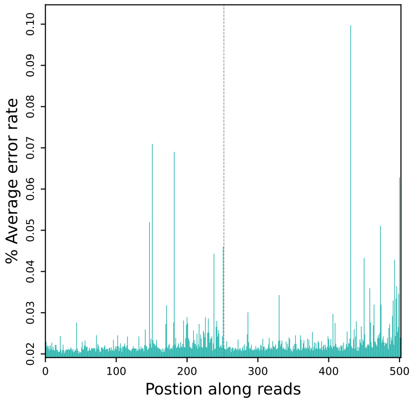
Error rate distribution along reads (R10309)
